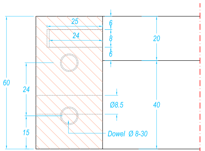
DETAIL #03 Scale 1 : 1
