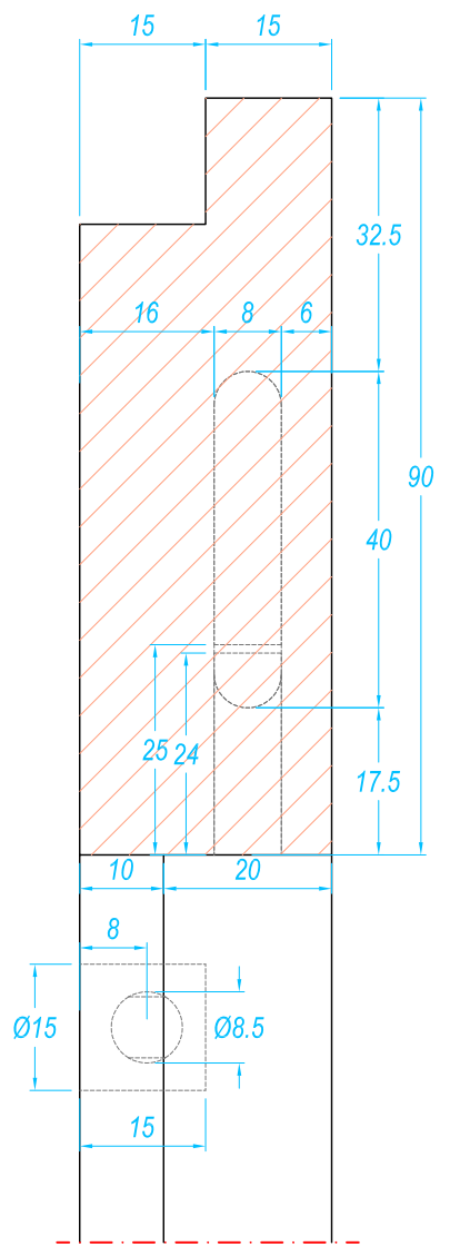
DETAIL #06 Scale 1 : 1
