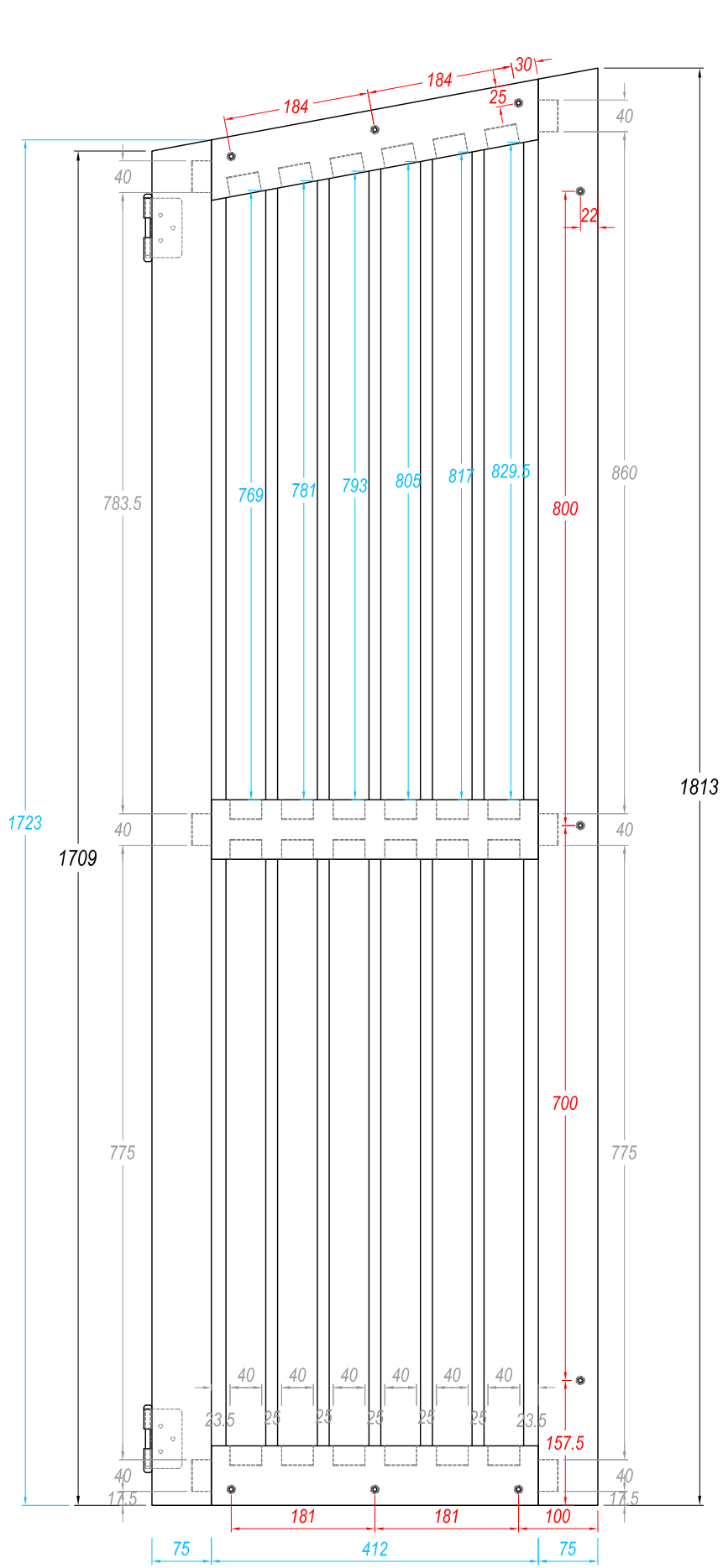
SIDE FRAME Scale 1 : 8
