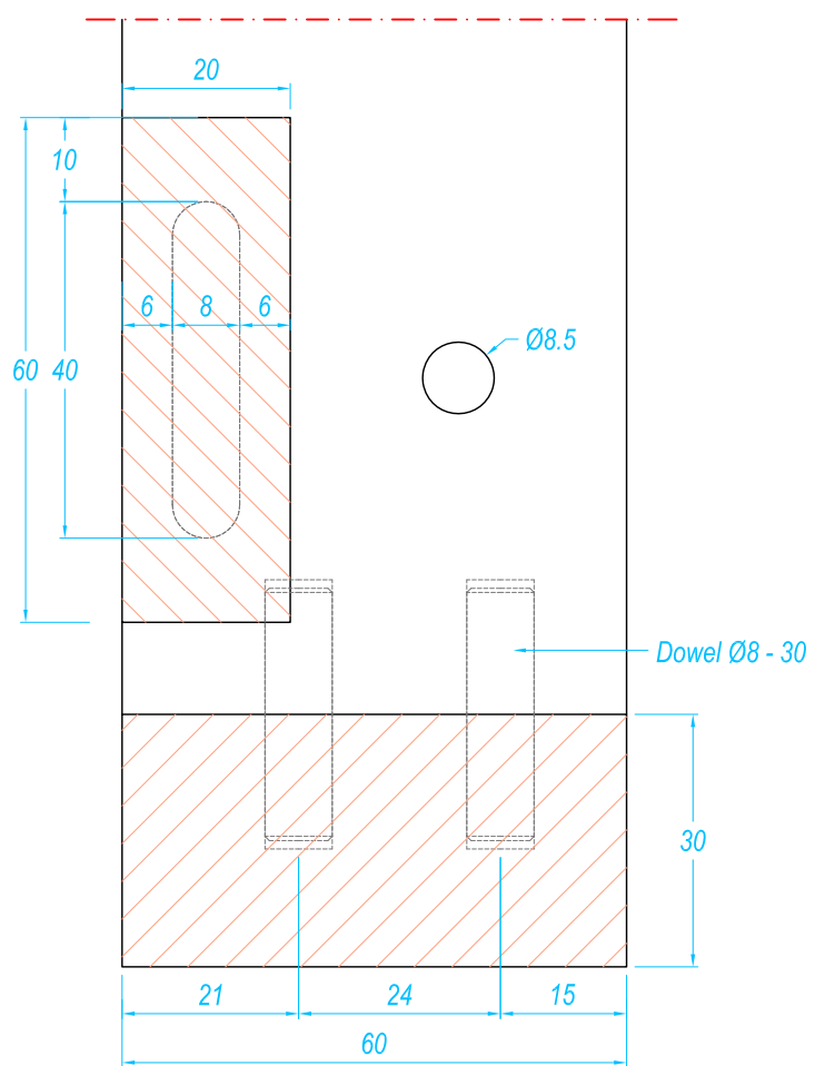
DETAIL #05 Scale 1 : 1
