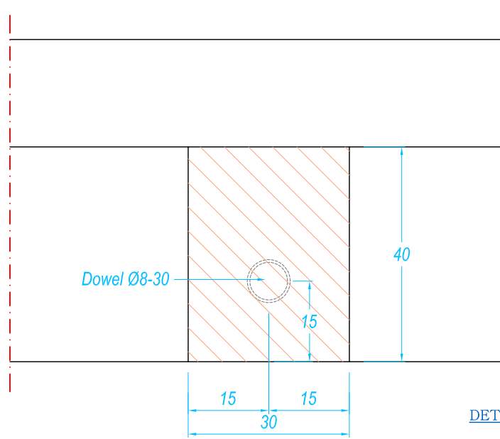
DETAIL #03 Scale 1 : 1
