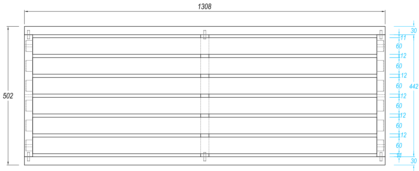
BASE FRAME Scale 1 : 8
