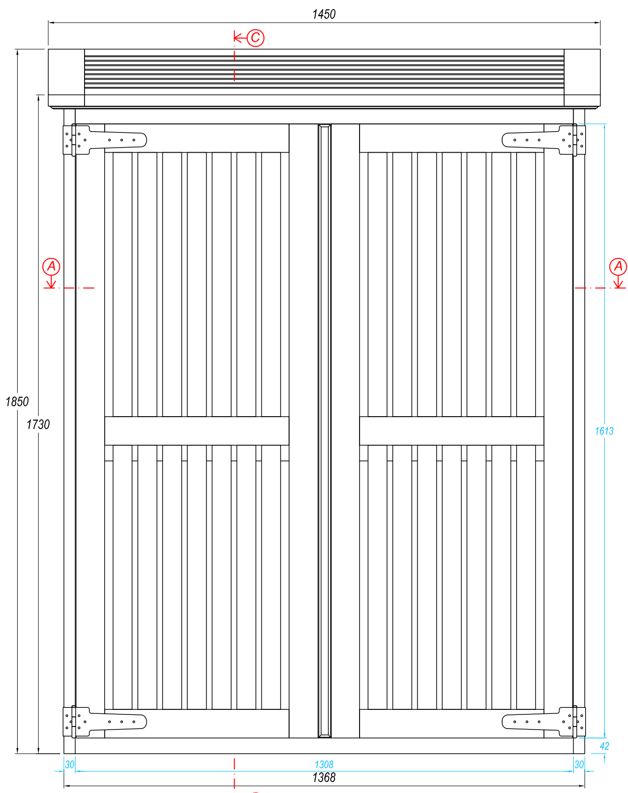
FRONT VIEW Scale 1 : 10
