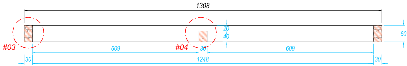
BASE FRAME Scale 1 : 8
