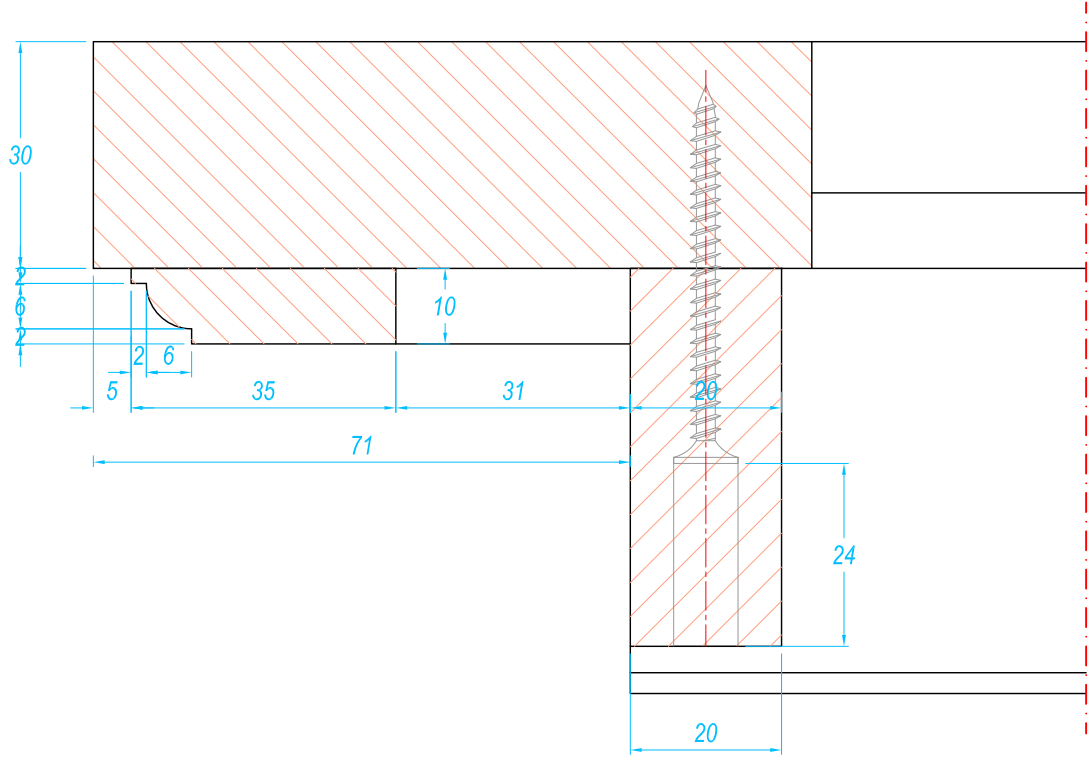
DETAIL #09 Scale 1 : 1
